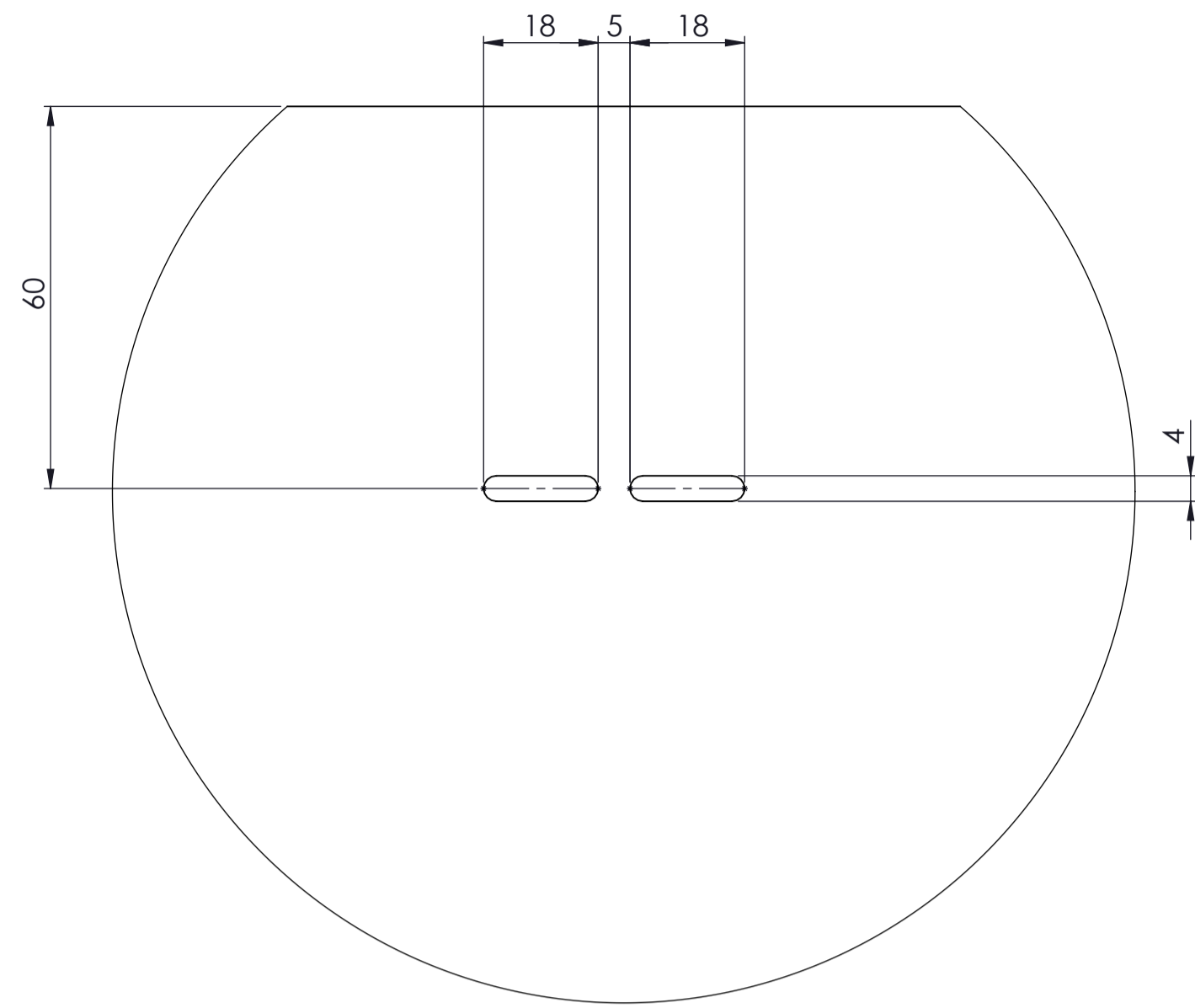
DETAIL A
