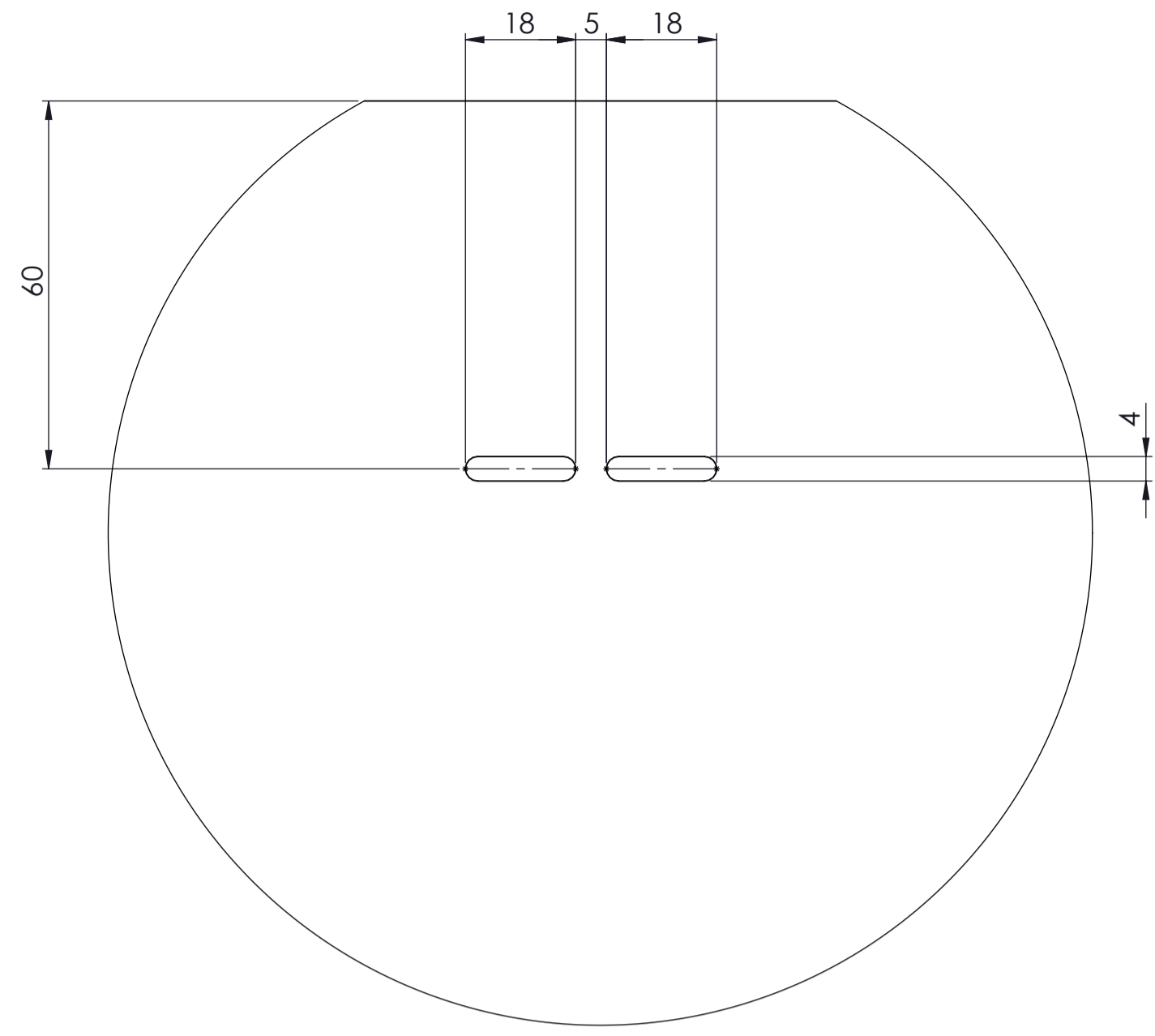
DETAIL A
