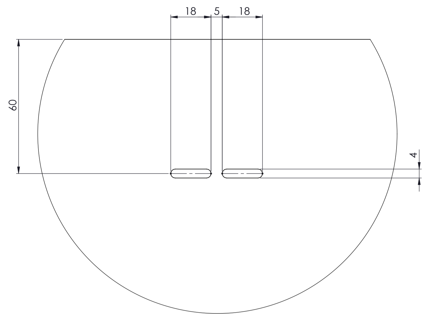
DETAIL A
