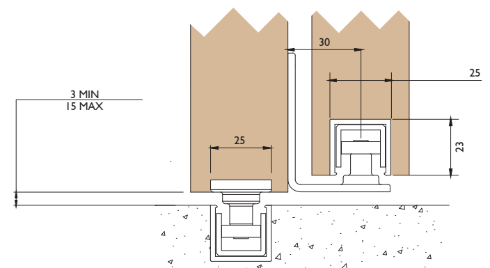
Detail 106HSS - 102SS/94 - 94SC + 94P
