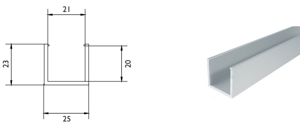
Detail 106SS/94 - 94SC + 94P
